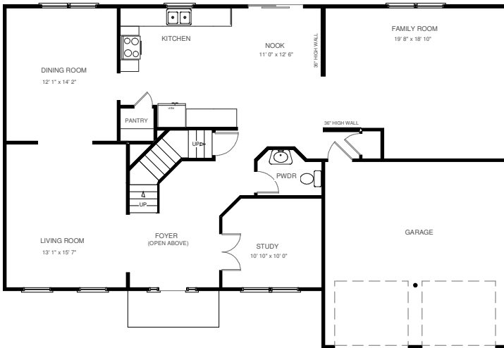
HANCOCK MODEL 2012 First Floor Plan
