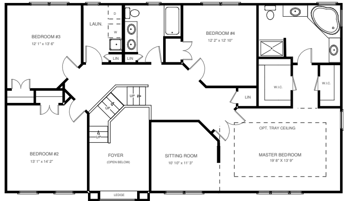
HANCOCK MODEL 2012 Second Floor Plan
